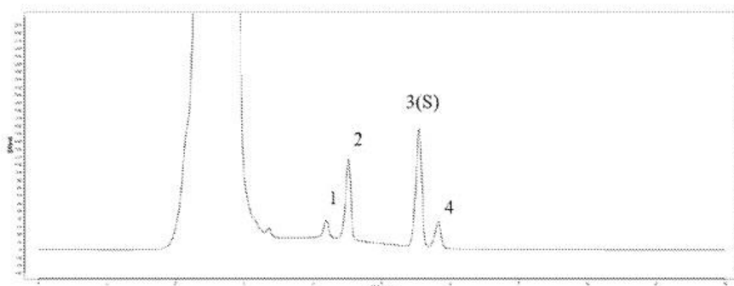
峰1: 槟榔次碱 峰3(S): 槟榔碱
