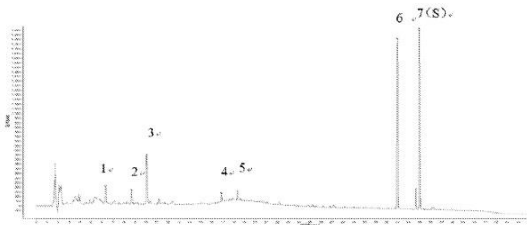
峰6: 和厚朴酚 峰7(S): 厚朴酚
